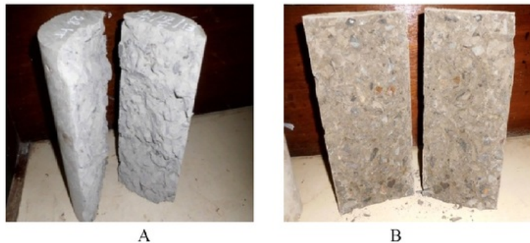
Fig. 5. Cylinder concrete with organic cement from tensile splitting test (A). Cylinder concrete with portland cement from tensile splitting test (B).
